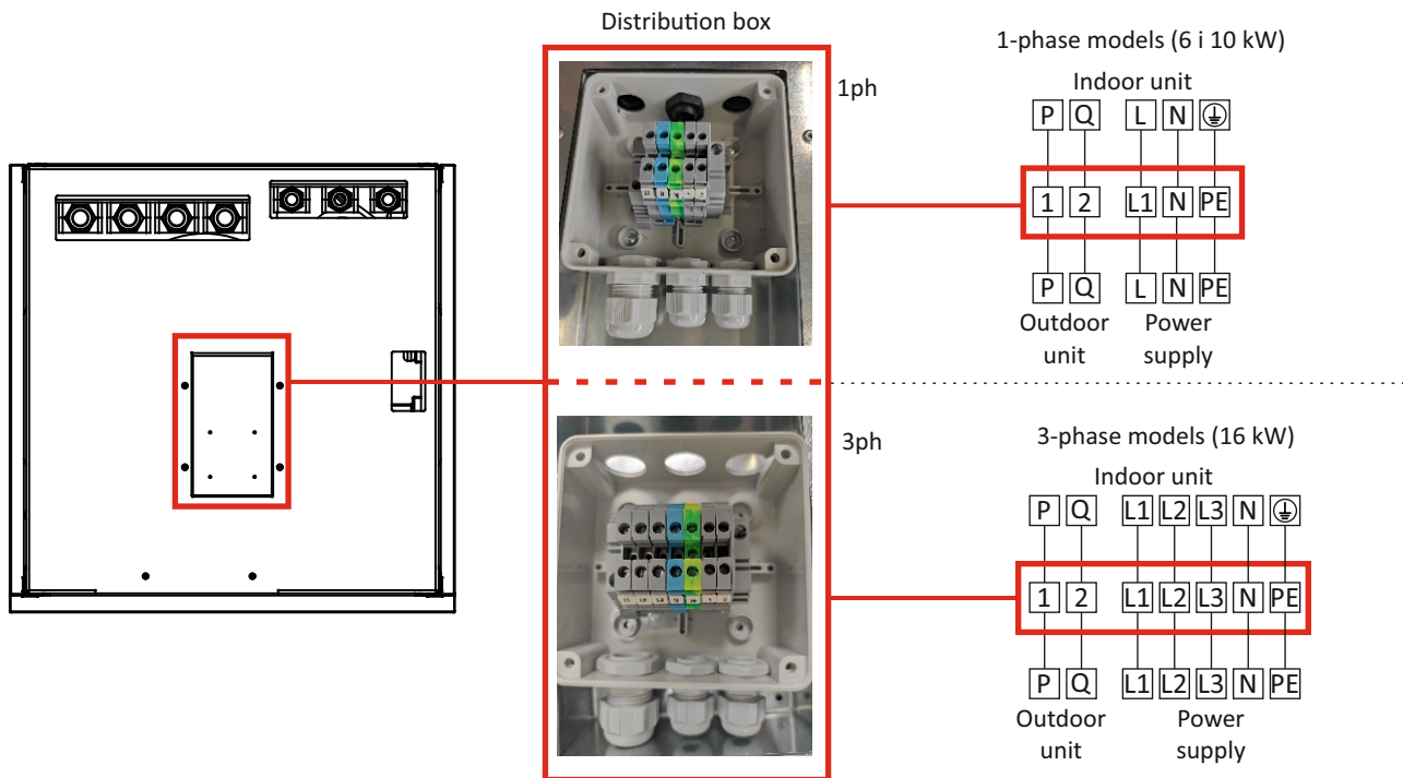
Figure 4.1: Indoor unit wiring diagram
