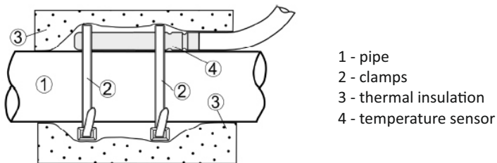
Figure 5.5: Additional circuit temperature sensor installation
