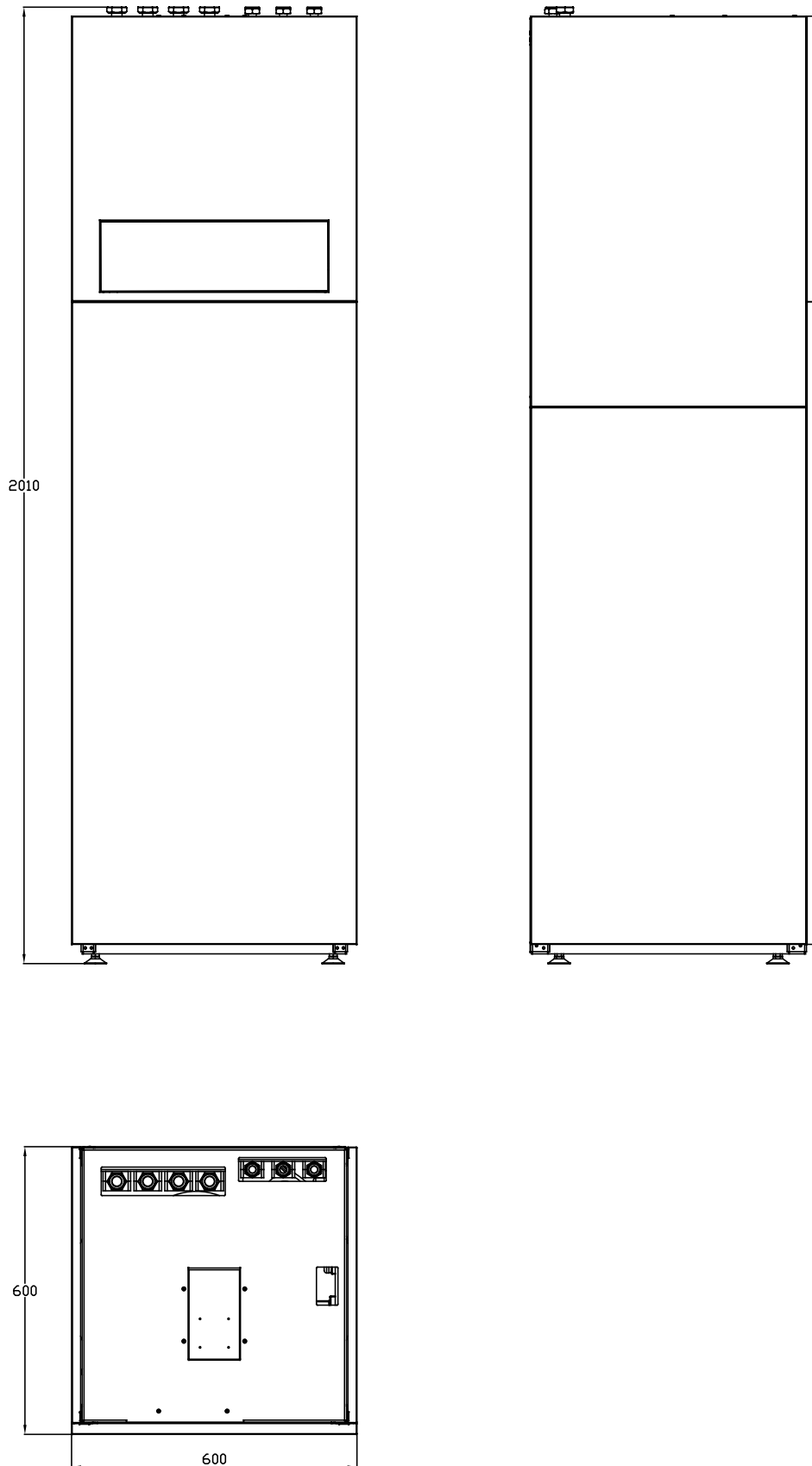
Figure 3.4: SHPAI60(100,160)RP24CM-EHT170 dimensions (unit: mm)
