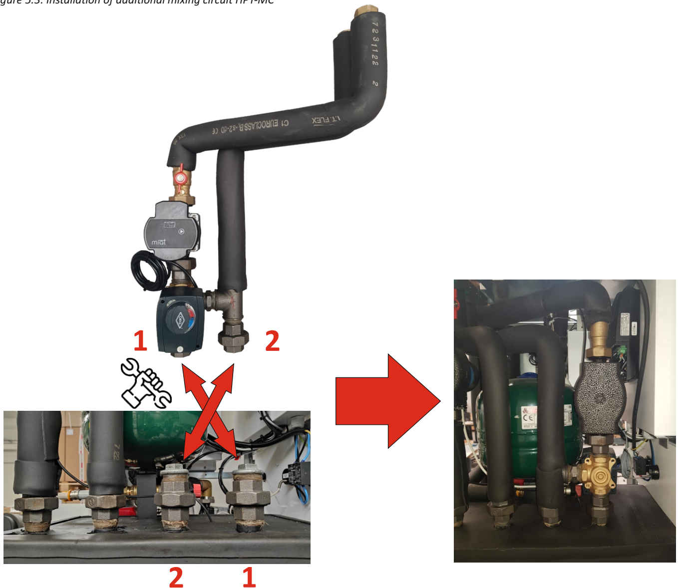
Figure 5.3: Installation of additional mixing circuit HPT-MC
