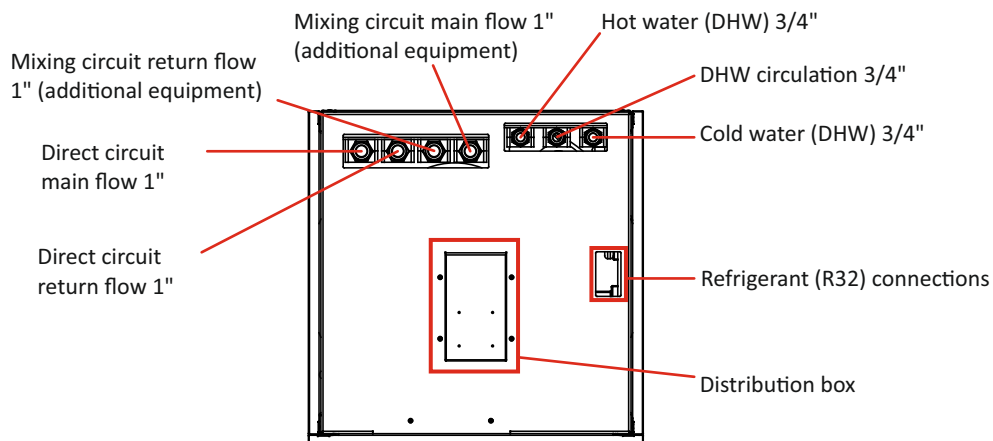
Figure 5.2: Tower heat pump top view with labeled connections
