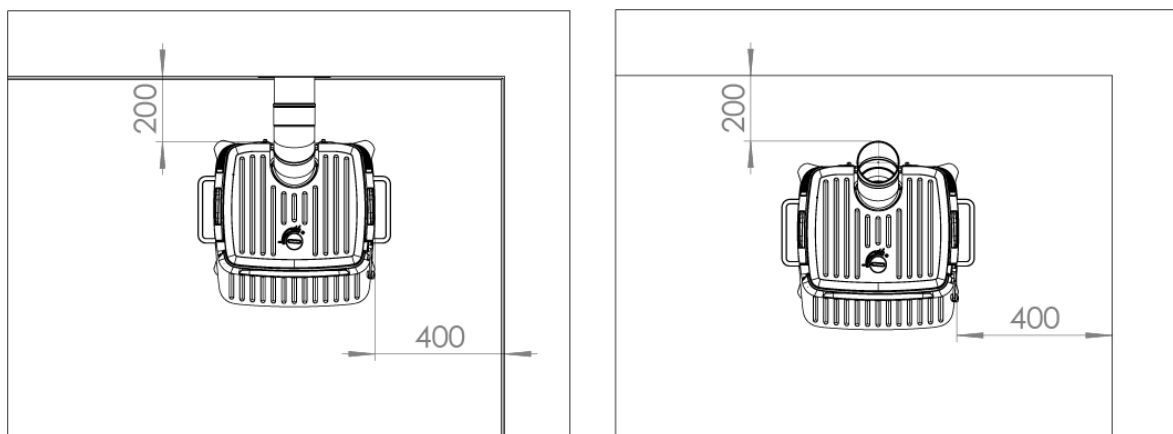
Figure 3 (Clearance from non-combustible material)
