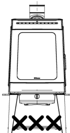
Figure 2 (Clearance from combustible material)
